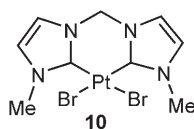
Figure 8. Platinum(II) complex 10 .
