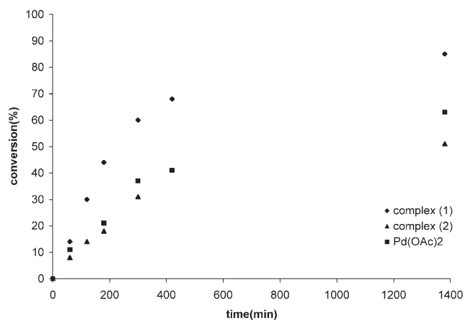
Figure 3. Conversion (%) vs. time diagram for the reaction of pentamethylbenzene and ethyl propiolate catalysed by complex 1 , complex 2 and Pd(OAc) 2 .
