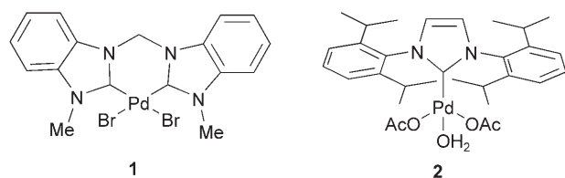
Figure 1. Complexes 1 and 2 .
