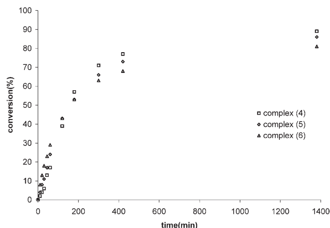
Figure 6. Conversion (%) vs. time diagram for the reaction of pentamethylbenzene and ethyl propiolate catalysed by complexes 4–6 .
