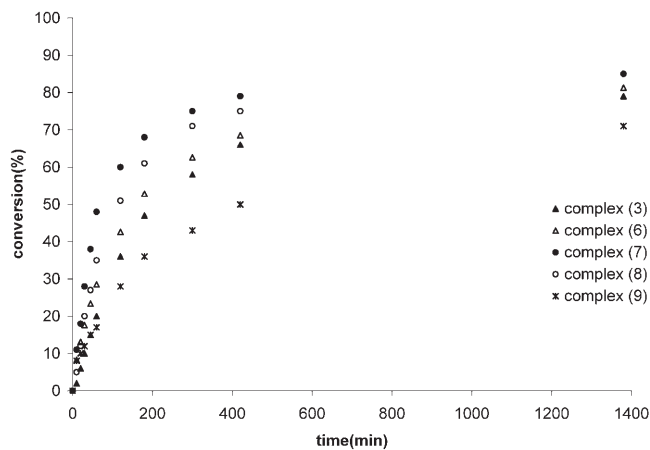
Figure 7. Conversion (%) vs. time diagram for the reaction of pentamethylbenzene and ethyl propiolate catalysed by complex 3 and complexes 6–9 .
