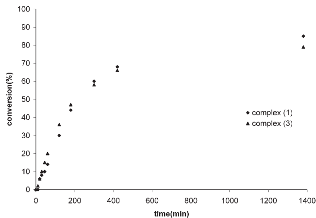
Figure 5. Conversion (%) vs. time diagram for the reaction of pentamethylbenzene and ethyl propiolate catalysed by complexes 1 and 3 .
