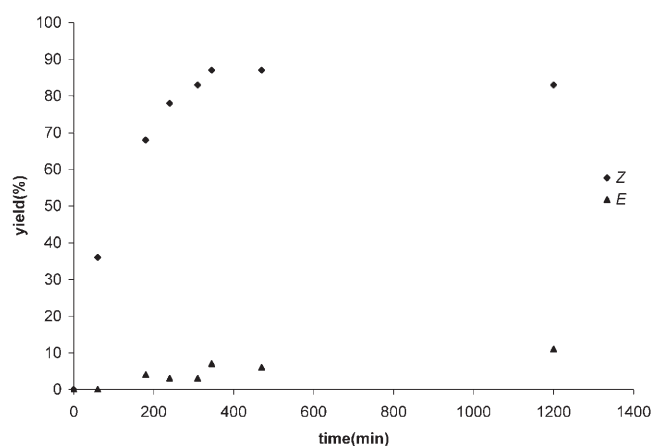
Figure 2. Yield (%) vs. time diagram for the reaction of pentamethylbenzene and ethyl propiolate catalysed by complex 1 .
